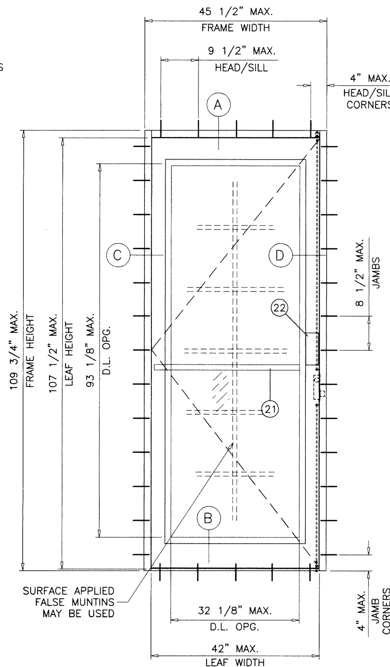
TYPICAL ELEVATION
